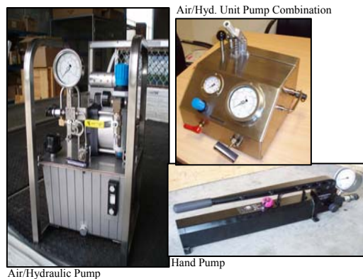
Air/Hydraulic Pump
